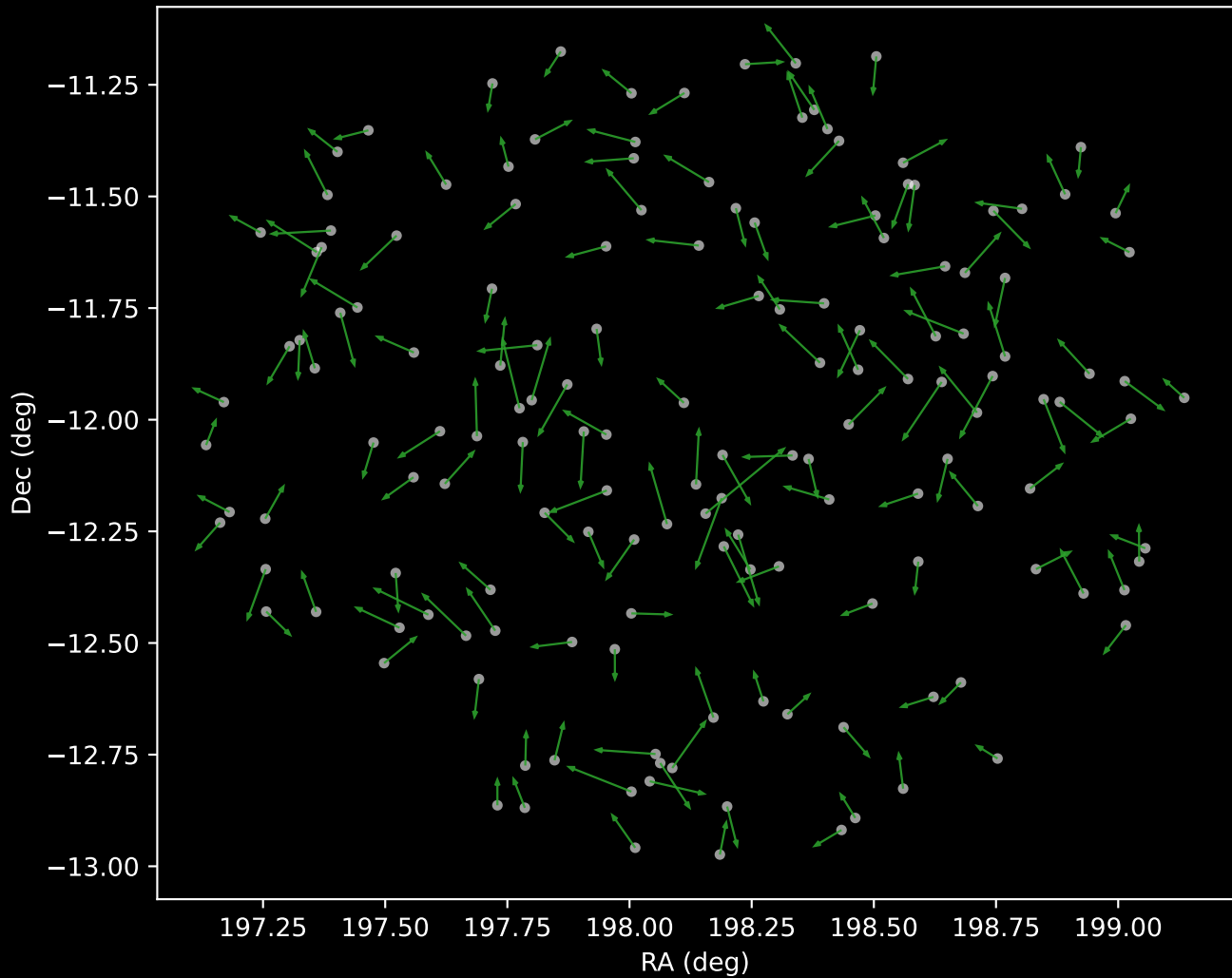
GALAH DR4 Cluster 4 Proper Motion Vectors (n=156)
