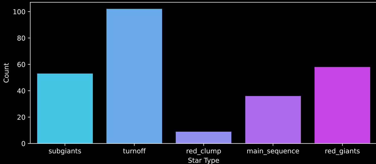
GALAH DR4 Field: [8823] Count plot of Star Type
